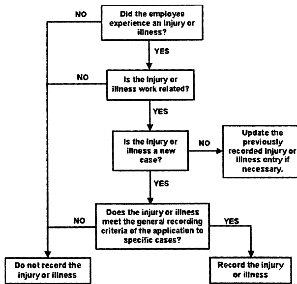
Decision Tree
