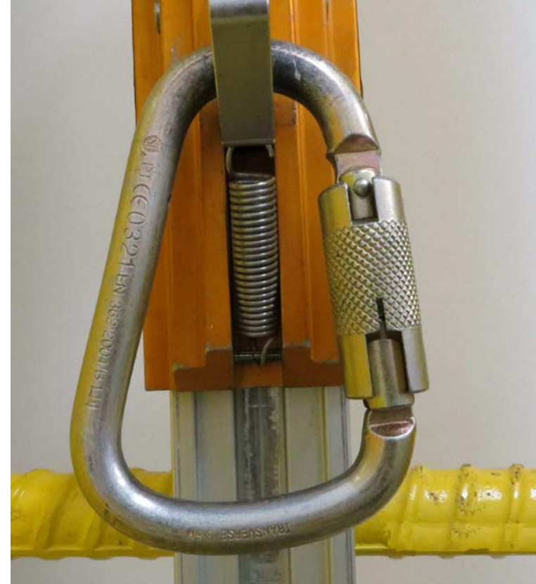
Photo 5. Locking carabiner to which the climber can directly connect the front waist D-ring of their full body harness..
